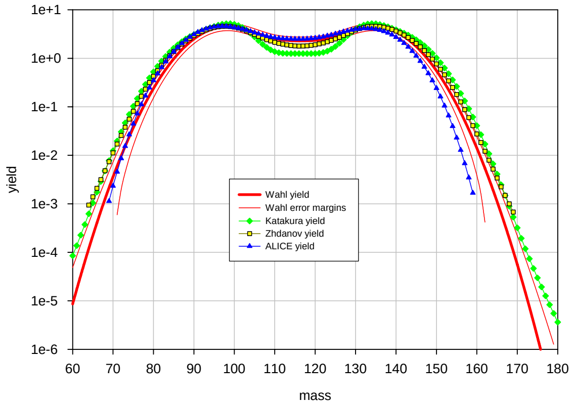
Benchmark B: ^{237}\text{Np} 28 MeV: post-neutron emission yields
